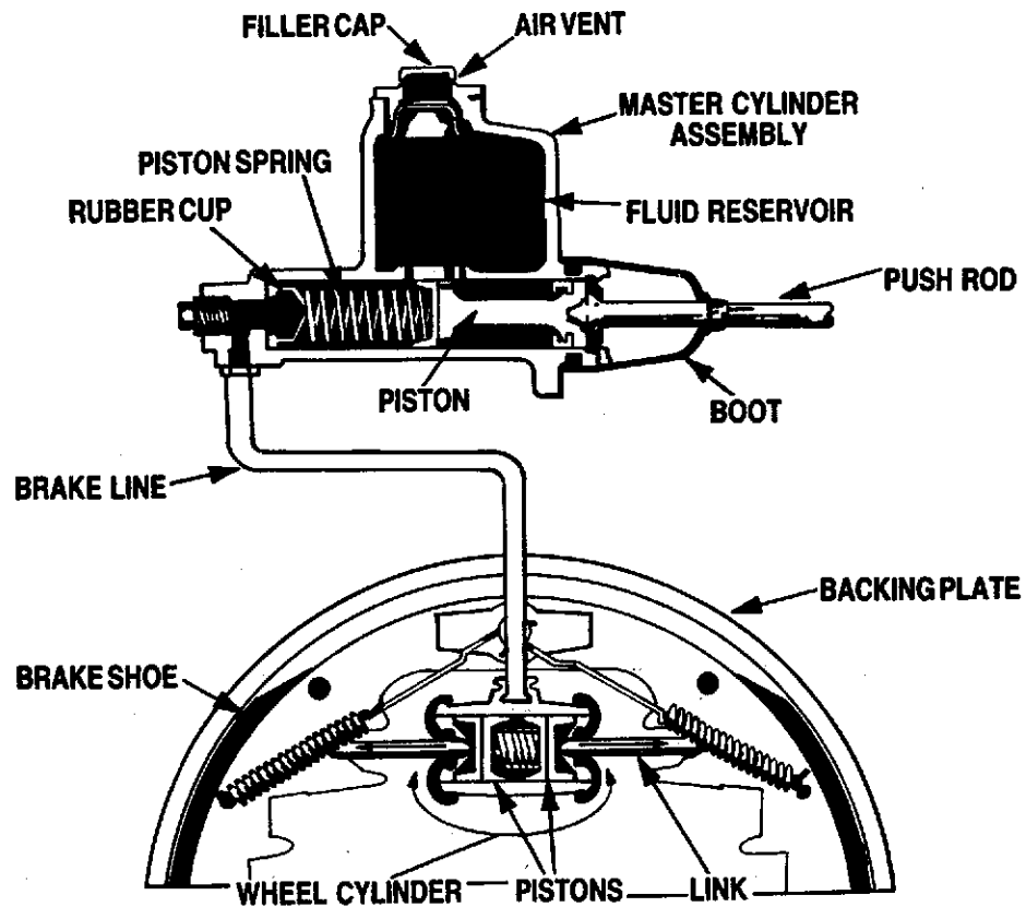
HYDRAULIC BRAKE SYSTEM
